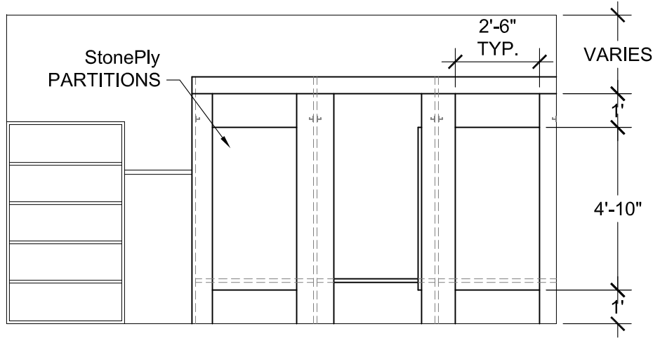
ELEVATION A 1/4" = 1'-0"
