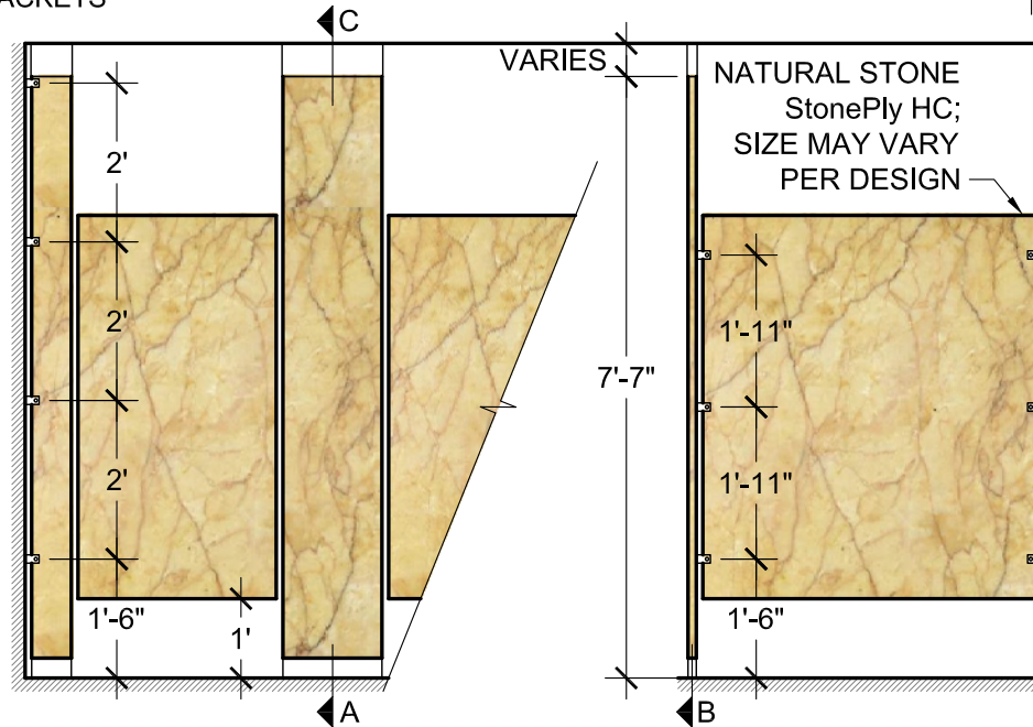
LAVATORY PARTITION ELEVATIONS SCALE: 3/8" = 1'
