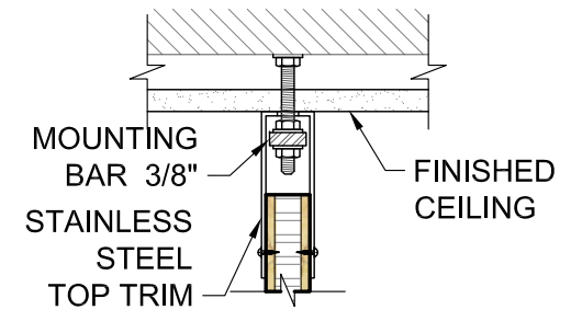
LAVATORY PARTITION CEILING DETAIL C SCALE: 2" = 1'
