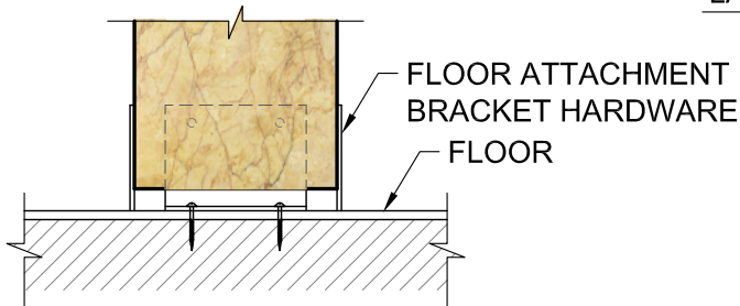
LAVATORY PARTITION FLOOR DETAIL B SCALE: 2" = 1'
