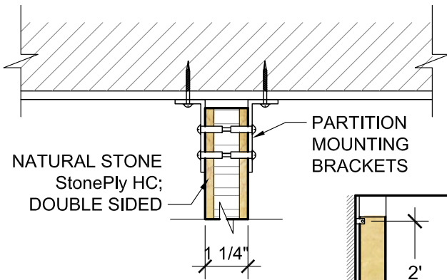
LAVATORY PARTITION WALL DETAIL SCALE: 3" = 1'
