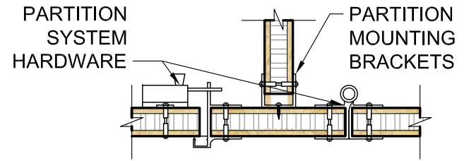
LAVATORY PARTITION DETAIL SCALE: 2" = 1'
